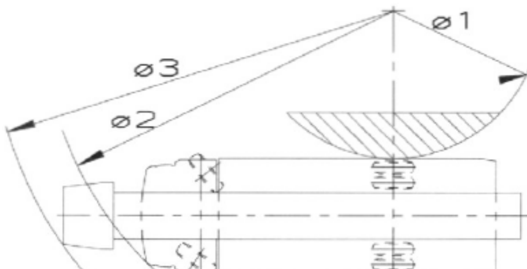
Figur 2: Svingradius stigebil
