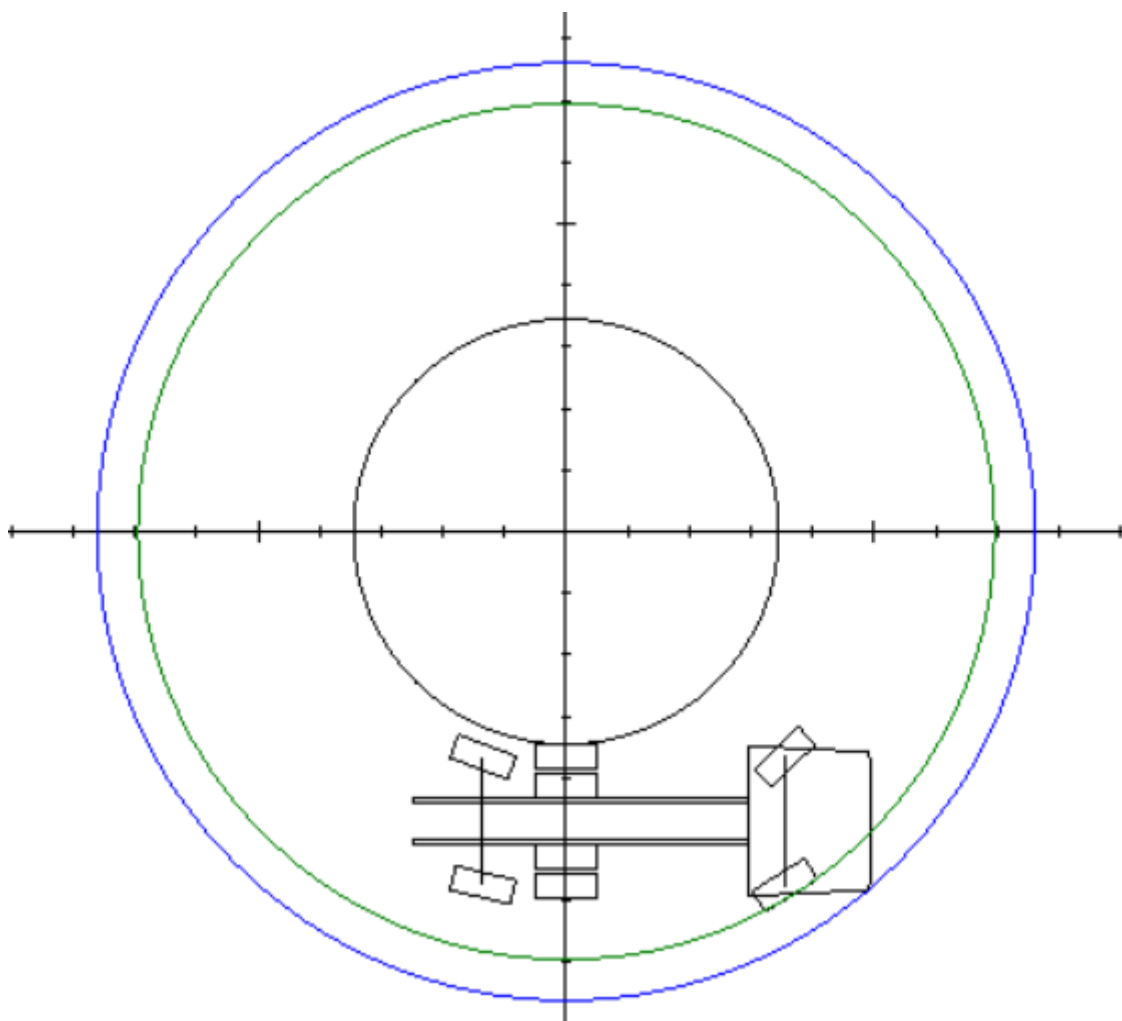
Figur 4: Svingradius tankbil
