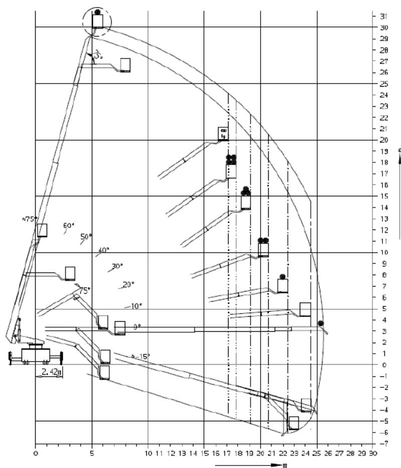
Figur 7: Rekkeviddediagram for stigebil
